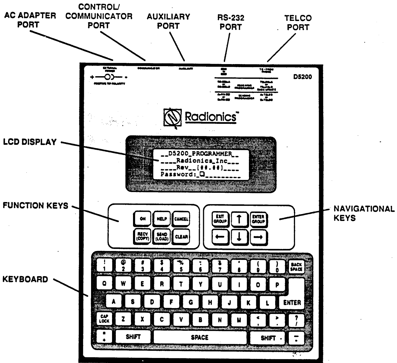
Figure 1: D5200 PROGRAMMER
