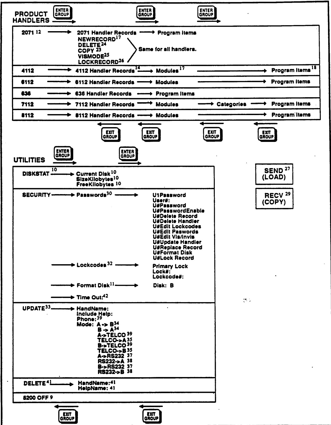
Figure 3: PROGRAMMER LEVELS
