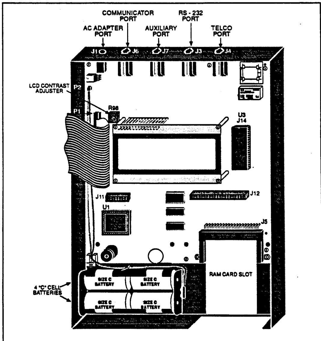
Figure 30: INSIDE THE PROGRAMMER
