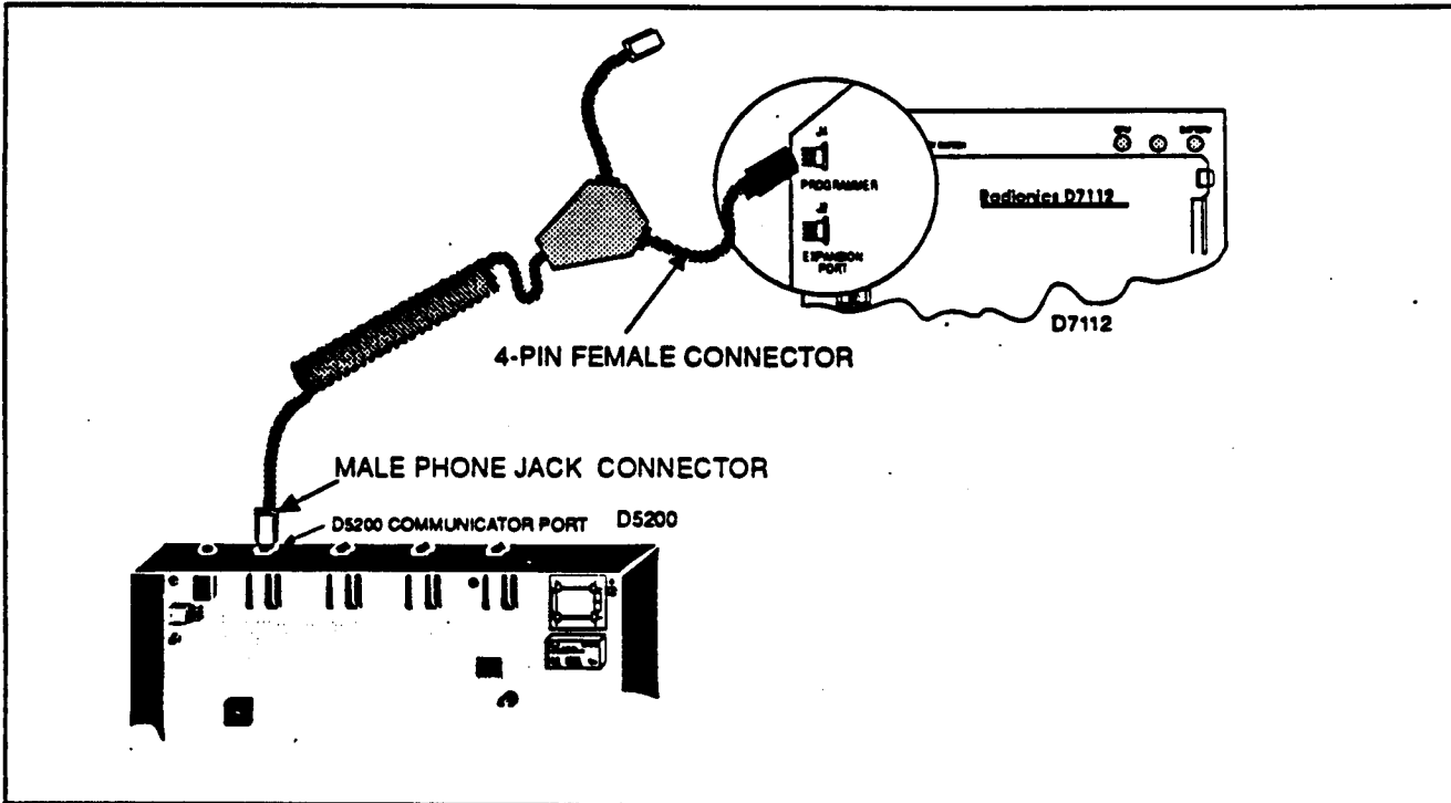
Figure 20: D5203 INTERFACE TO A PANEL WITH A MOLEX PROGRAMMER CONNECTOR
